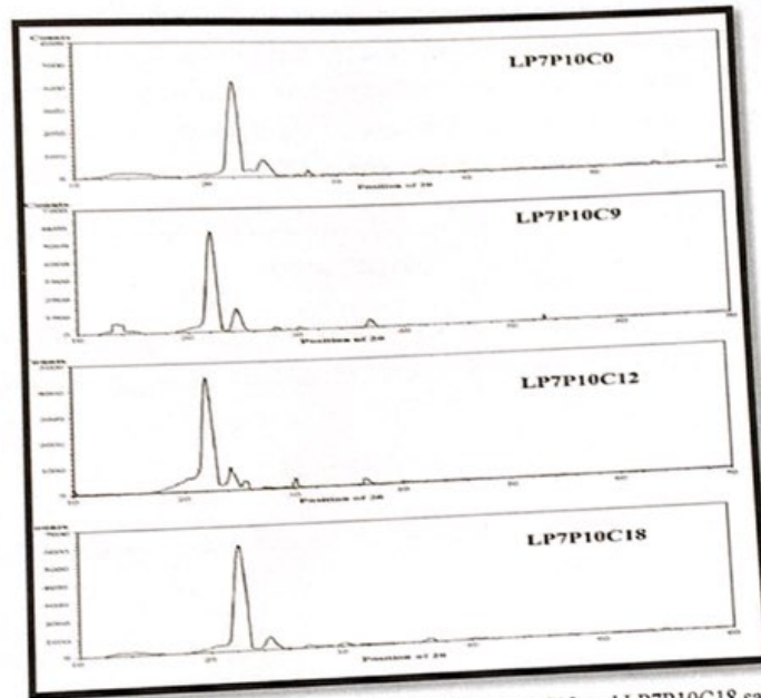
Figure 2: XRD patterns for LP7P10C0, LP7P10C9, LP7P10C12 and LP7P10C18 samples.
