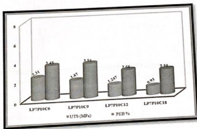
Figure 1: UTS and PEB values for LP7P10C0, LP7P10C9, LP7P10C12 and LP7P10C18 before and after degradation.
